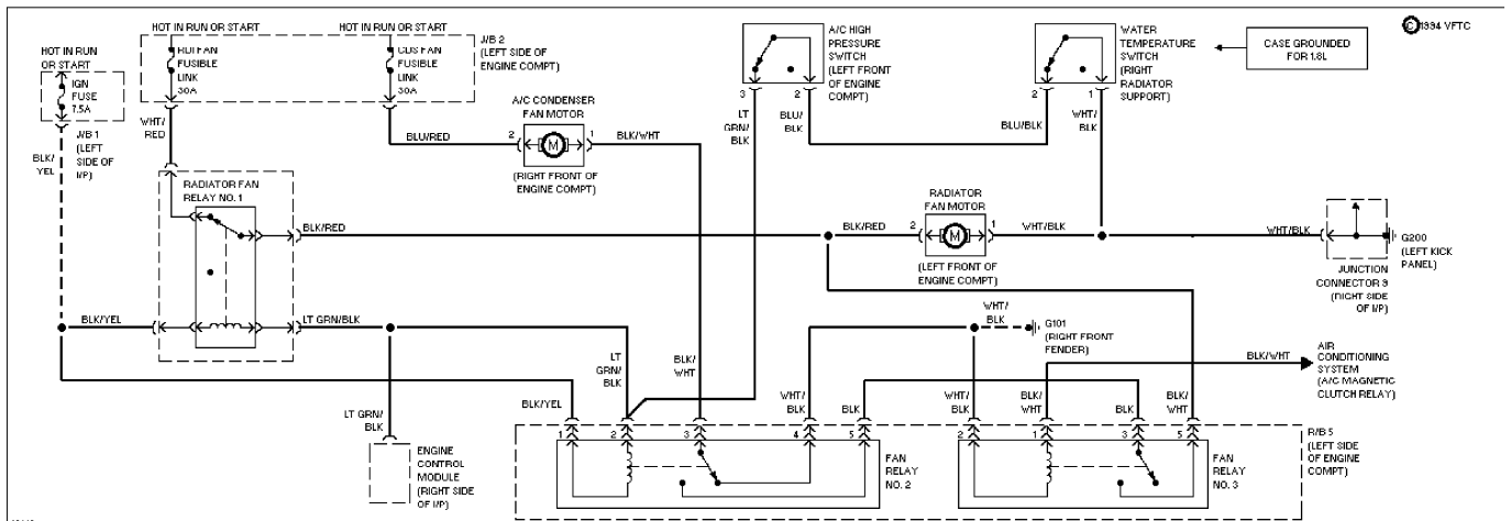
Fig. 5: Electric Cooling Fan Wiring Diagram
