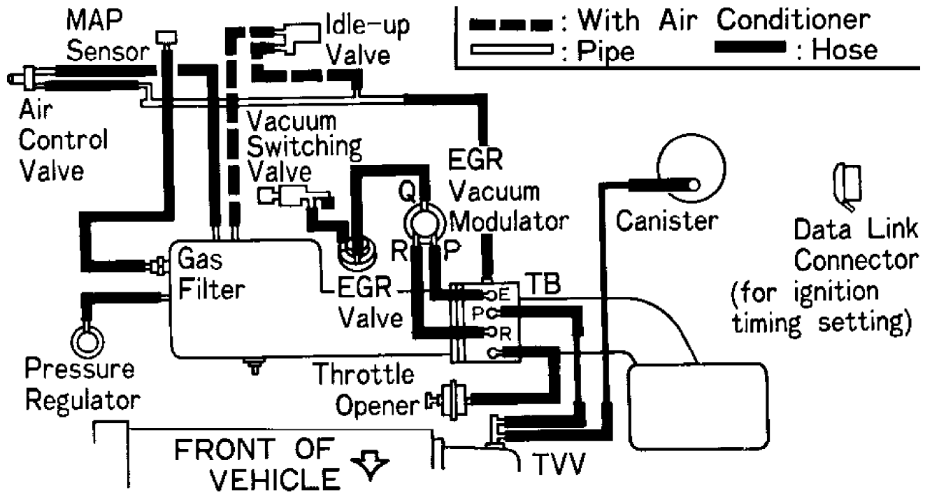
Fig. 1: Vacuum Diagram (1.8L 7A-FE) Courtesy of Toyota Motor Sales, U.S.A., Inc.
