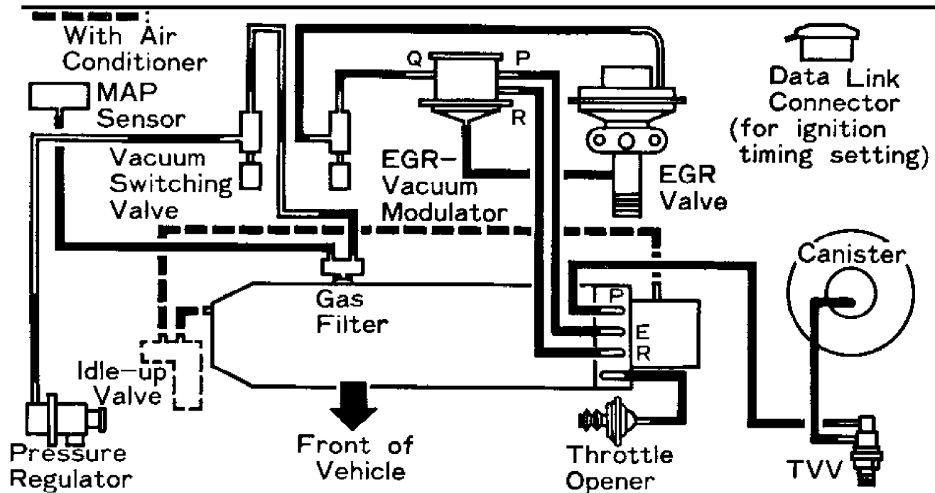
Fig. 3: Vacuum Diagram (2.2L 5S-FE - California) Courtesy of Toyota Motor Sales, U.S.A., Inc.
