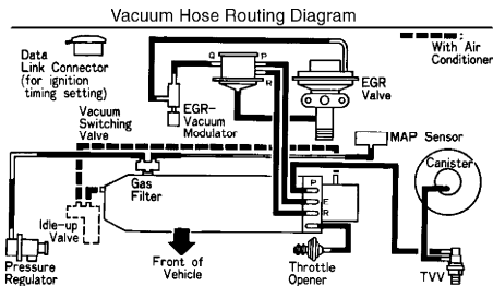
Fig. 2: Vacuum Diagram (2.2L 5S-FE - Federal) Courtesy of Toyota Motor Sales, U.S.A., Inc.
