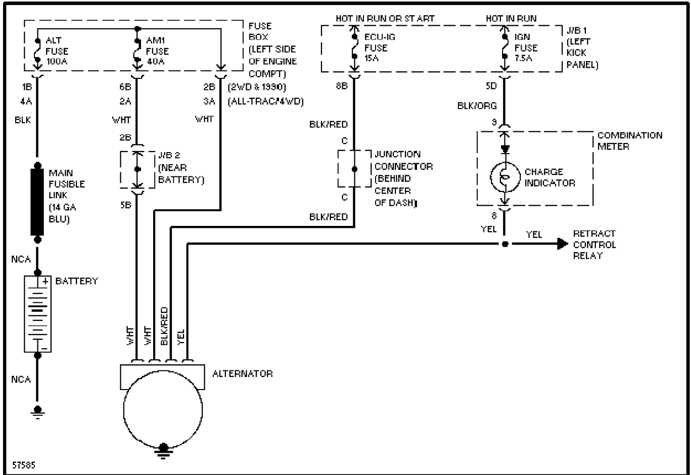
Charging Circuit
