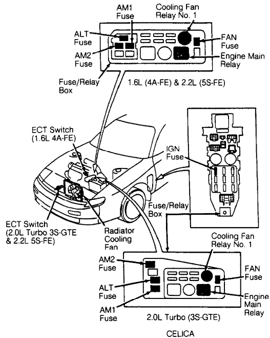
Fig. 1: Identifying Radiator Cooling Fan & Components Courtesy of Toyota Motor Sales, U.S.A., Inc.
