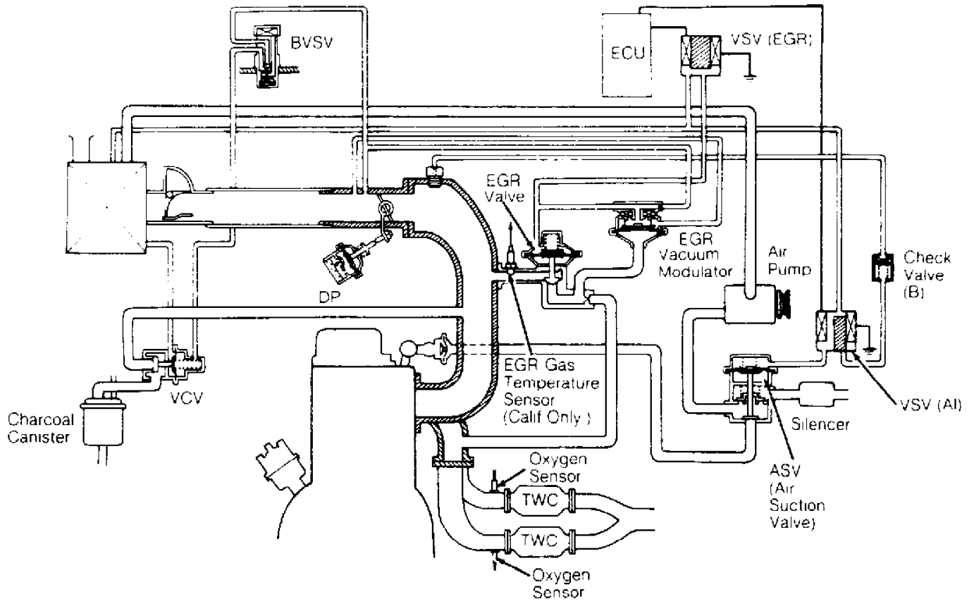
Fig. 13: Land Cruiser 4.1L Courtesy of Toyota Motor Sales, U.S.A., Inc.
