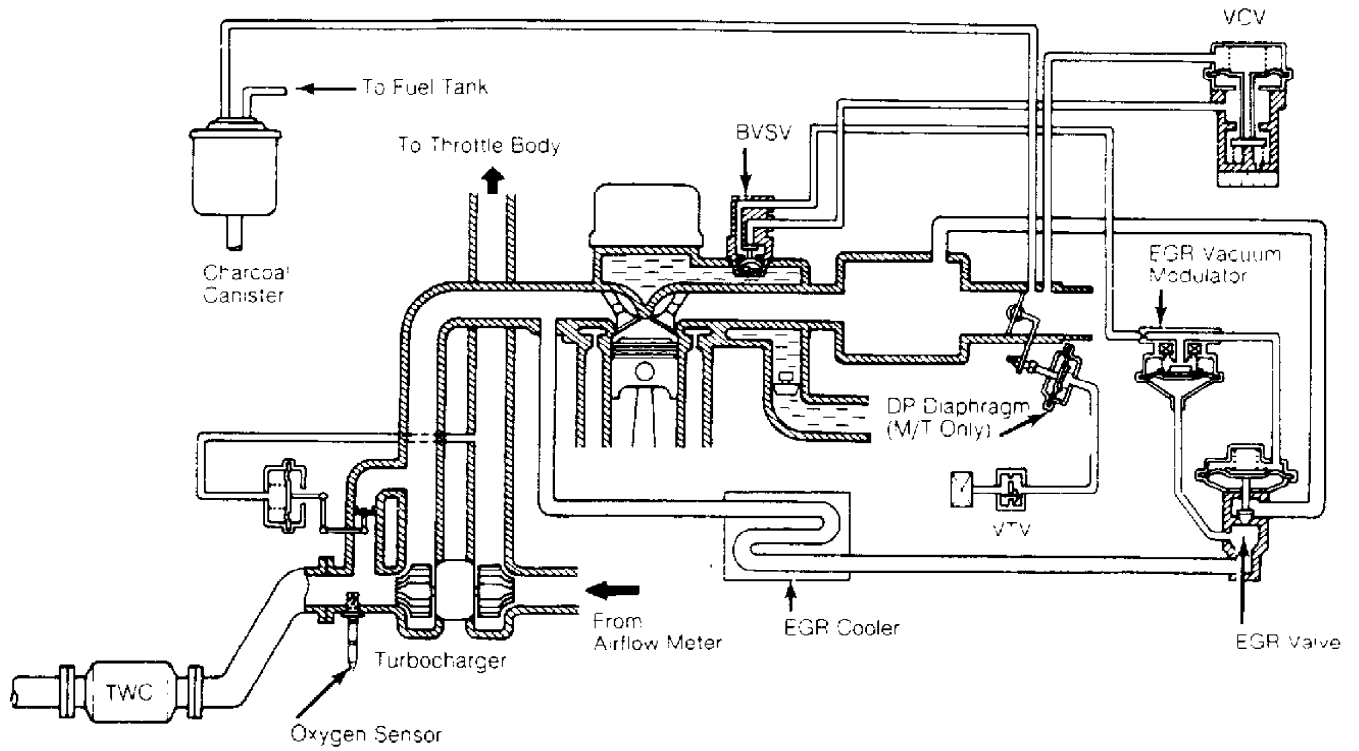
Fig. 17: Pickup & 4Runner 2.4L (EFI, Turbo) Courtesy of Toyota Motor Sales, U.S.A., Inc.
