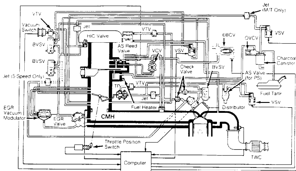
Fig. 21: Tercel 1.5L (California) Courtesy of Toyota Motor Sales, U.S.A., Inc.
