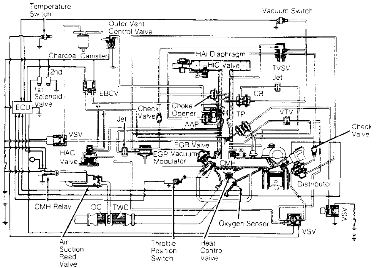
Fig. 9: Corolla 1.6L FX (Carbureted/Federal with A/T) Courtesy of Toyota Motor Sales, U.S.A., Inc.
