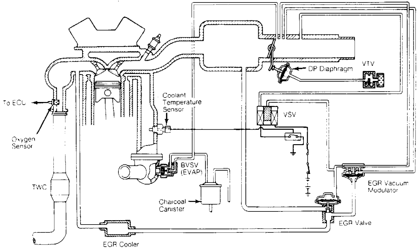
Fig. 12: Cressida 2.8L Courtesy of Toyota Motor Sales, U.S.A., Inc.
