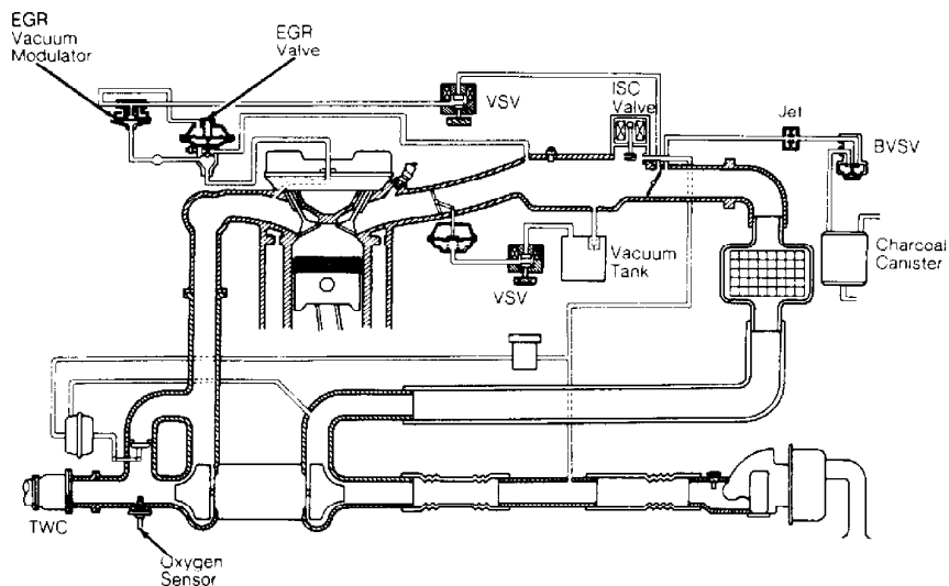
Fig. 4: Celica (All-Trac 4WD) Courtesy of Toyota Motor Sales, U.S.A., Inc.
