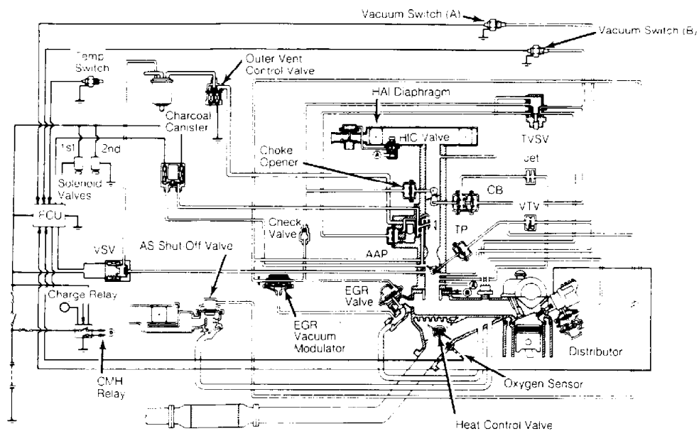
Fig. 23: Tercel Wagon 1.5L (California) Courtesy of Toyota Motor Sales, U.S.A., Inc.
