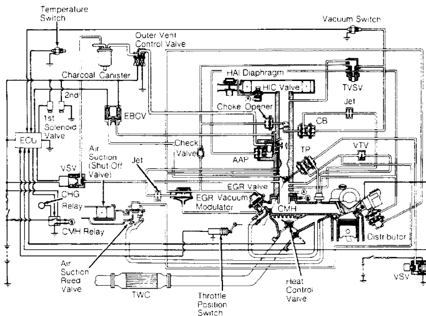
Fig. 10: Corolla 1.6L FX (Carbureted/California with M/T) Courtesy of Toyota Motor Sales, U.S.A., Inc.
