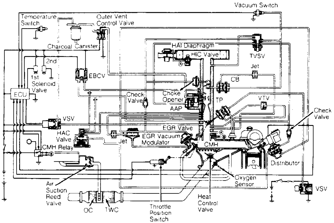
Fig. 11: Corolla 1.6L FX (Caarbureted/Federal with M/T) Courtesy of Toyota Motor Sales, U.S.A., Inc.
