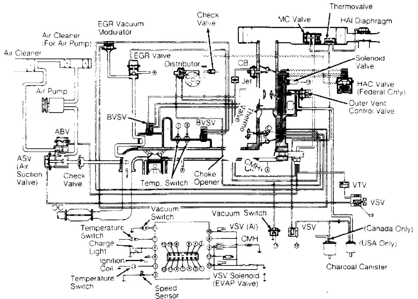
Fig. 15: Pickup 2.4L (Federal/Carbureted) Courtesy of Toyota Motor Sales, U.S.A., Inc.
