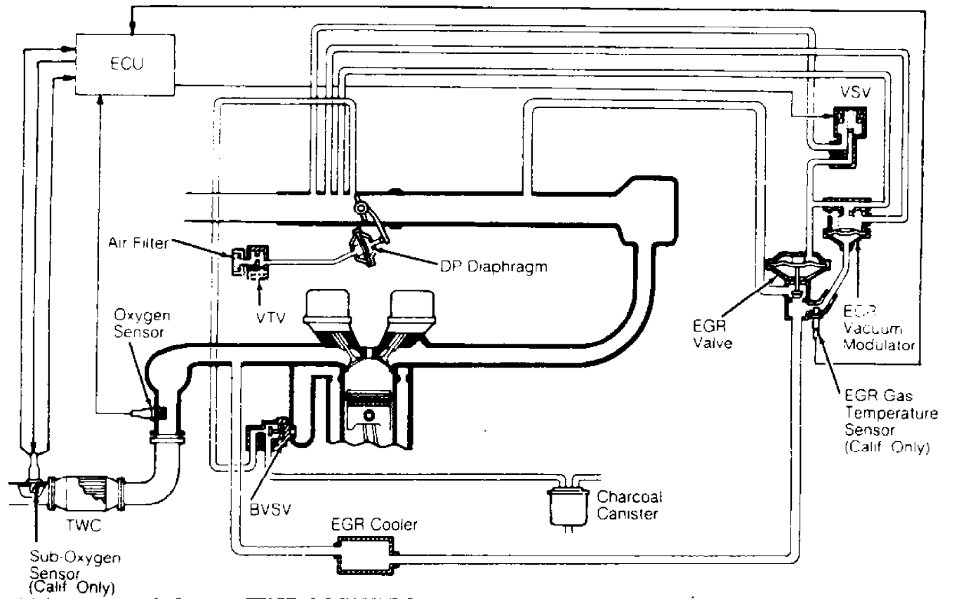
Fig. 19: Supra 3.0L (Non-Turbo) Courtesy of Toyota Motor Sales, U.S.A., Inc.
