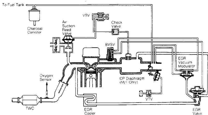
Fig. 16: Pickup-4Runner 2.4L (EFI, Non-Turbo) Courtesy of Toyota Motor Sales, U.S.A., Inc.
