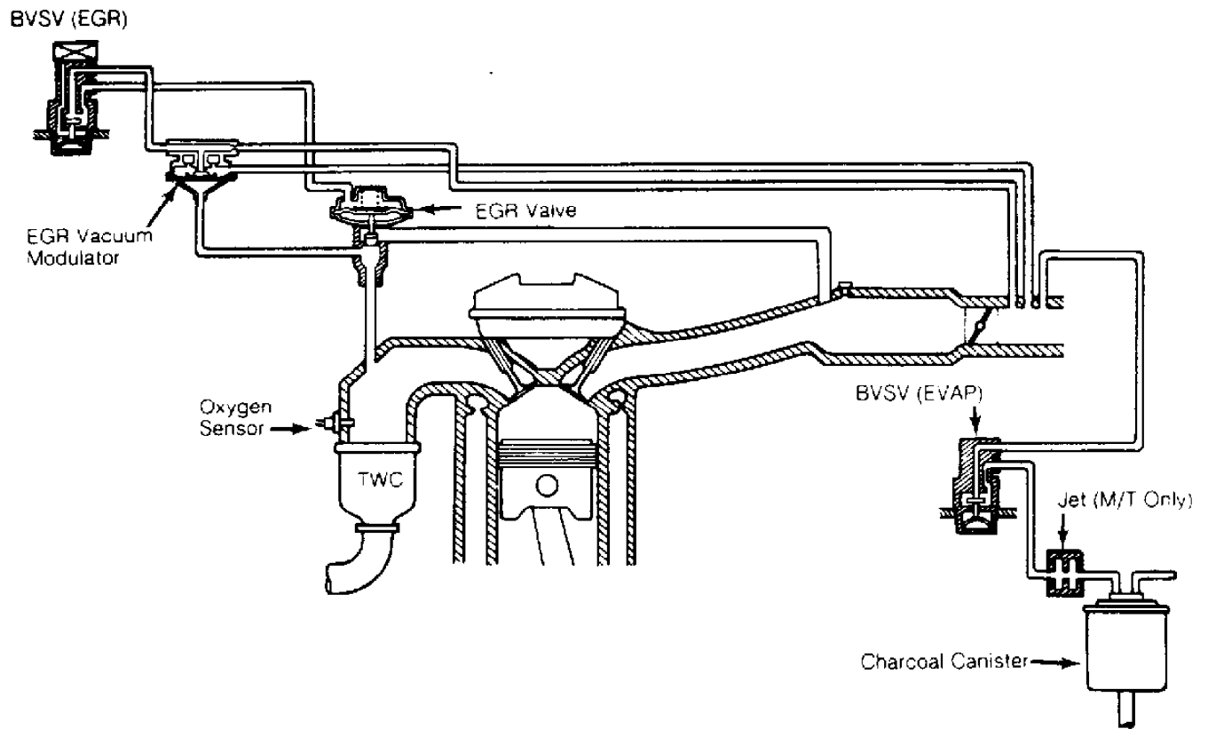
Fig. 1: Camry & Celica 2.0L Non-Turbo Courtesy of Toyota Motor Sales, U.S.A., Inc.
