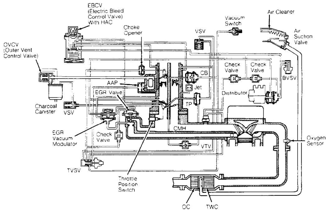
Fig. 6: Corolla a.6L (Federal / Carbureted) Courtesy of Toyota Motor Sales, U.S.A., Inc.
