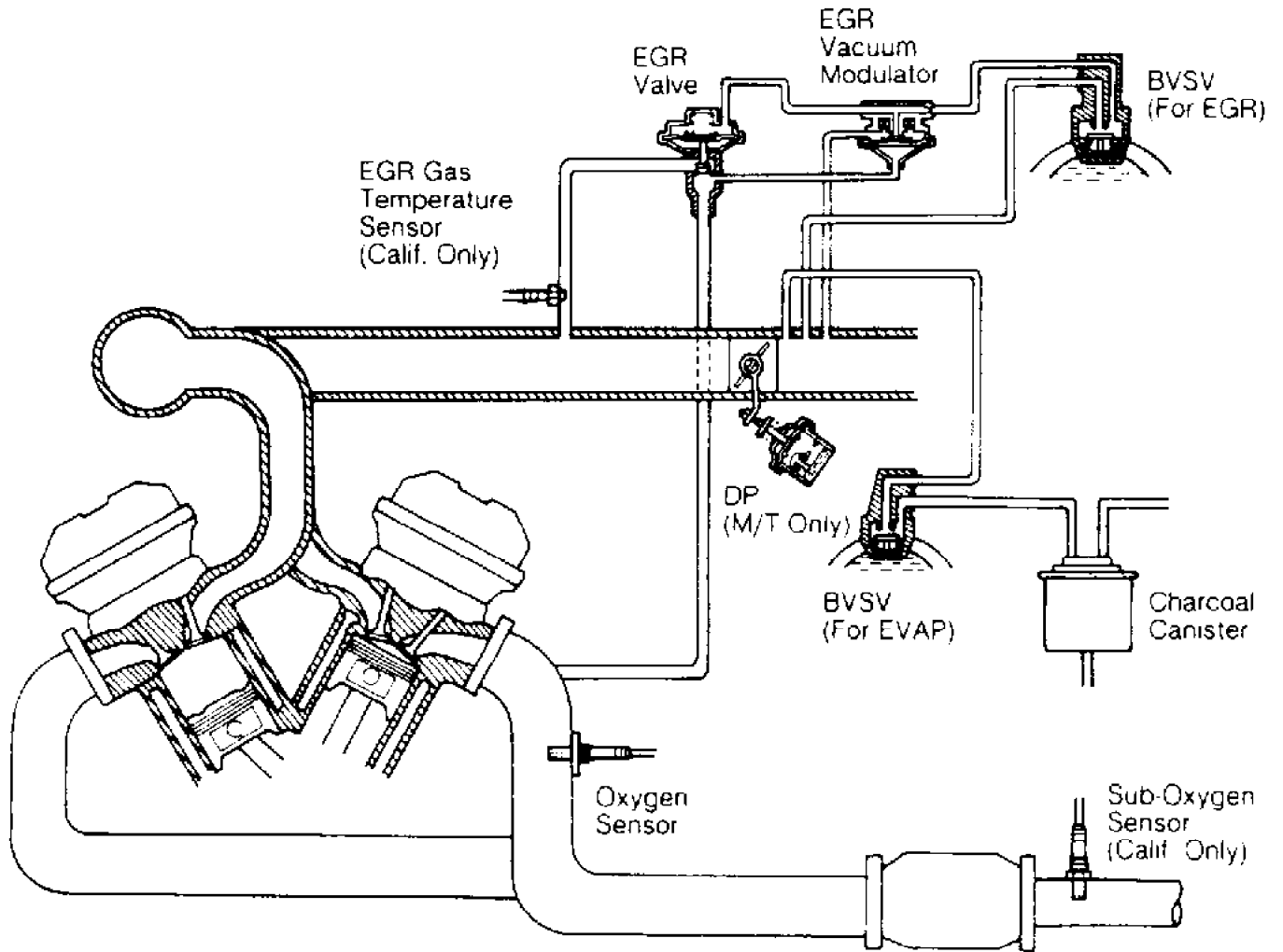
Fig. 2: 1988 1/2 Camry 2.5L V6 (VZV Series) Courtesy of Toyota Motor Sales, U.S.A., Inc.
