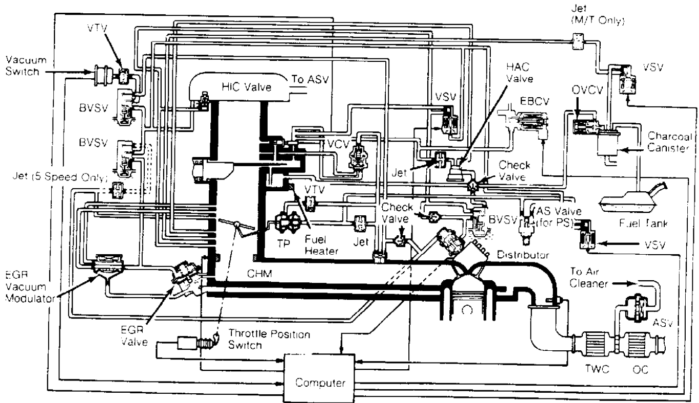
Fig. 22: Tercel 1.5L (Federal) Courtesy of Toyota Motor Sales, U.S.A., Inc.
