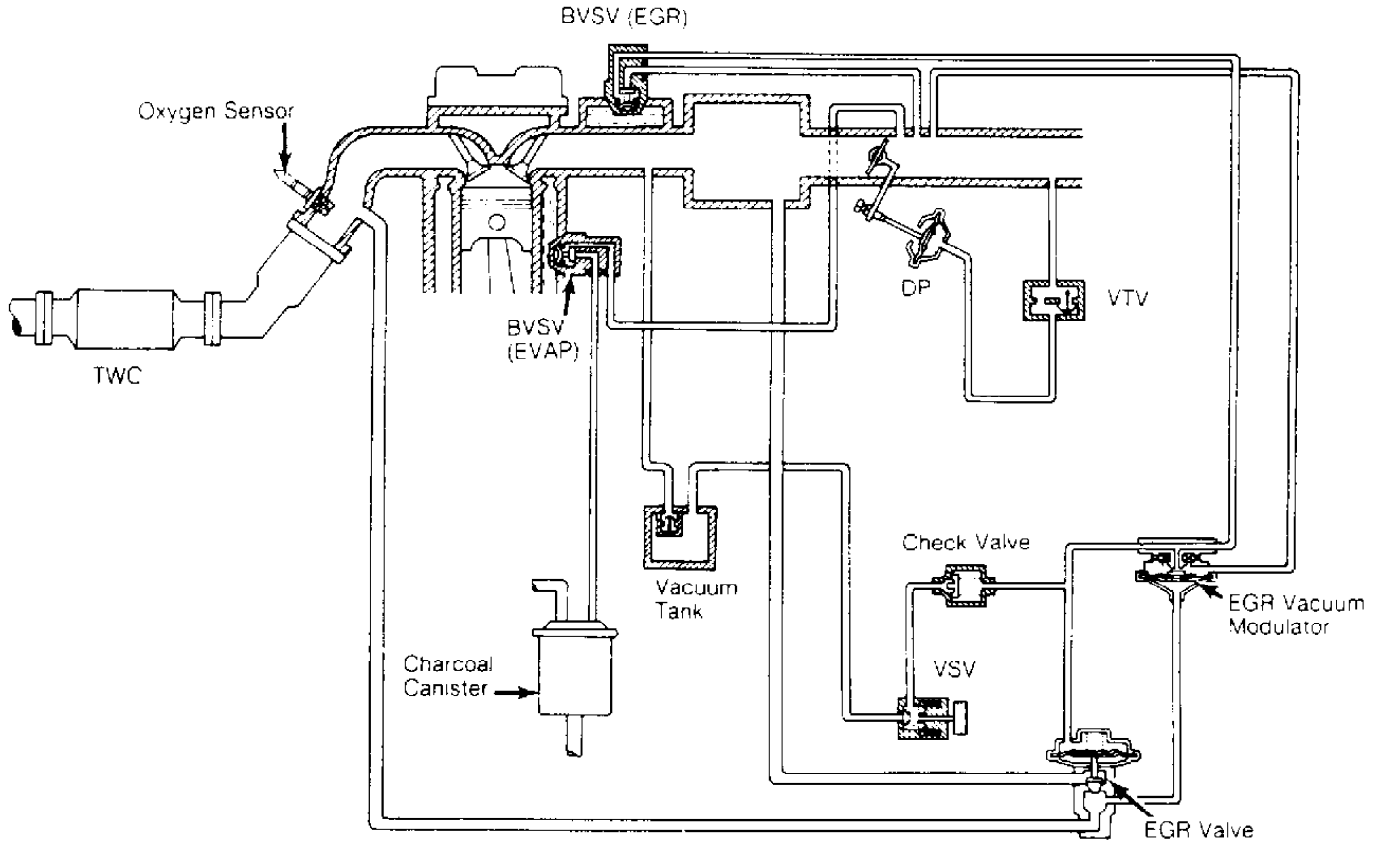
Fig. 7: Corolla 1.6L (EFI), FX, FX-16 (EFI) & MR2 Courtesy of Toyota Motor Sales, U.S.A., Inc.
