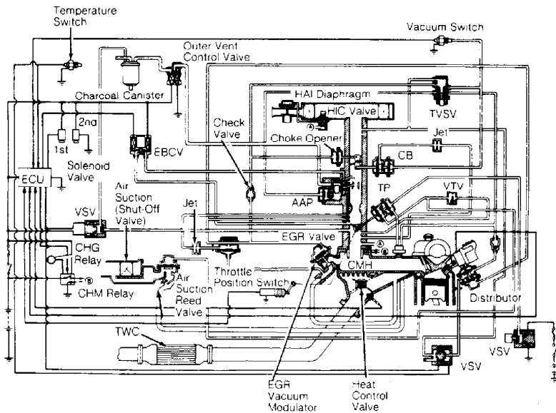
Fig. 8: Corolla 1.6L FX (Carbureted/California with A/T) Courtesy of Toyota Motor Sales, U.S.A., Inc.
