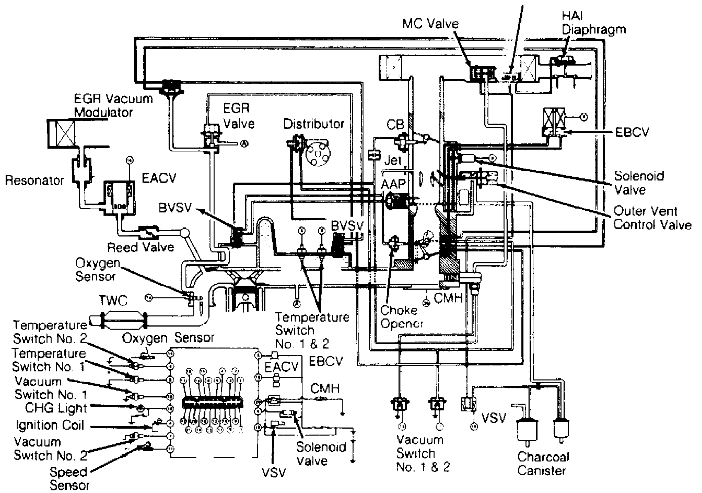
Fig. 14: Pickup 2.4L (California/Carbureted) Courtesy of Toyota Motor Sales, U.S.A., Inc.
