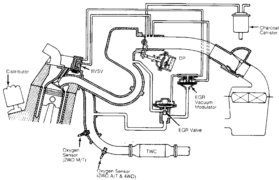
Fig. 25: Van 2.2L Courtesy of Toyota Motor Sales, U.S.A., Inc.
