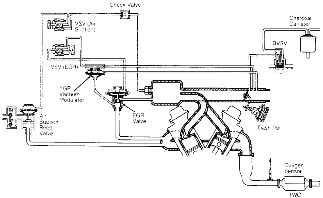
Fig. 18: Pickup & 4Runner .30L V6 (VZN Series) Courtesy of Toyota Motor Sales, U.S.A., Inc.
