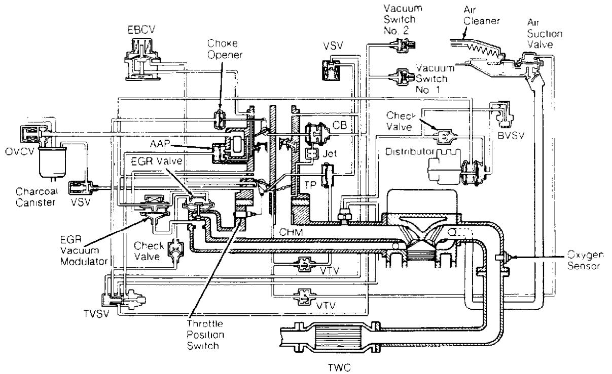
Fig. 5: Corolla 1.6L (California/ Carbureted) Courtesy of Toyota Motor Sales, U.S.A., Inc.
