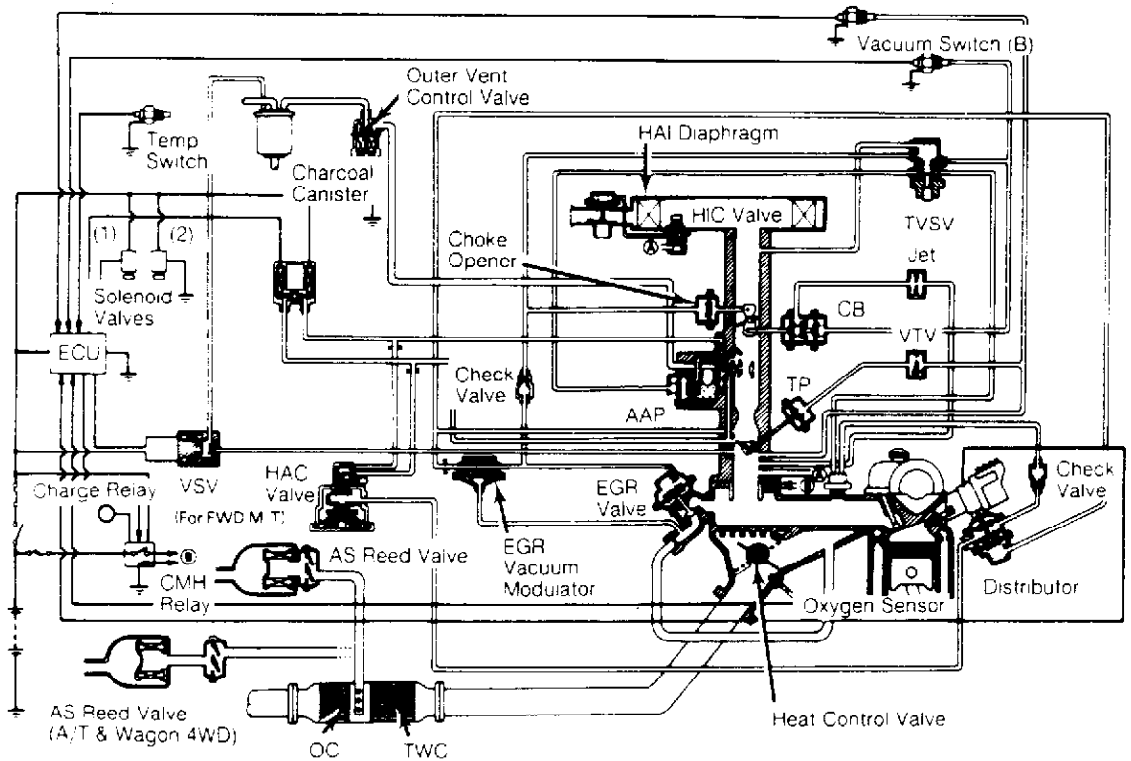
Fig. 24: Tercel Wagon 1.15L (Federal) Courtesy of Toyota Motor Sales, U.S.A., Inc.
